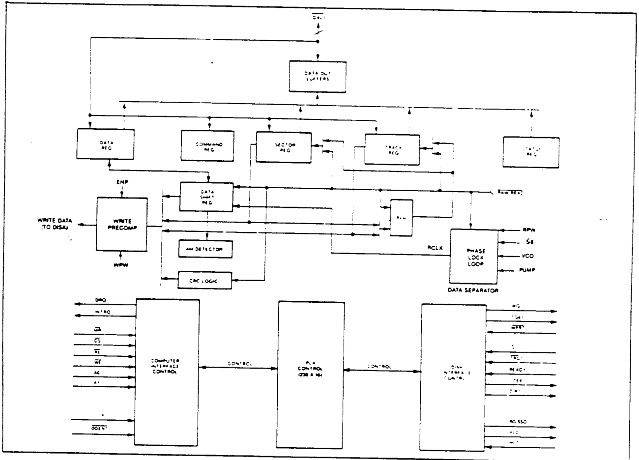
Figure 2. WD279X BLOCK DIAGRAM
