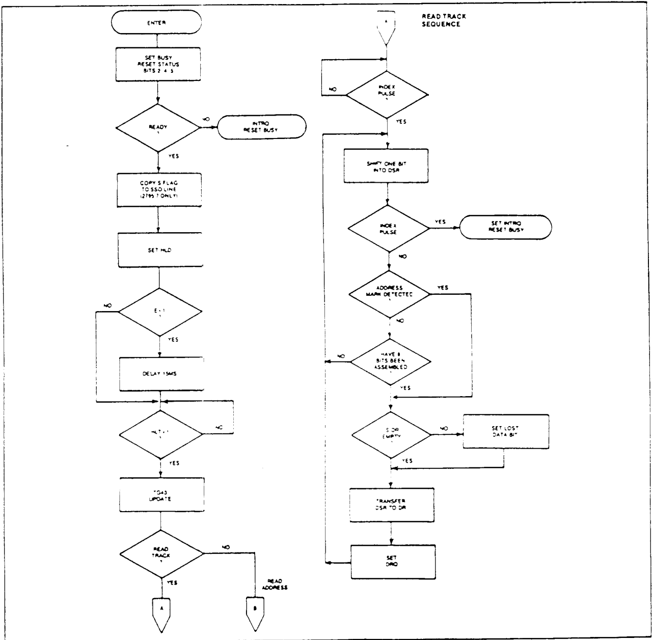
TYPE III COMMAND Read Track/Address
