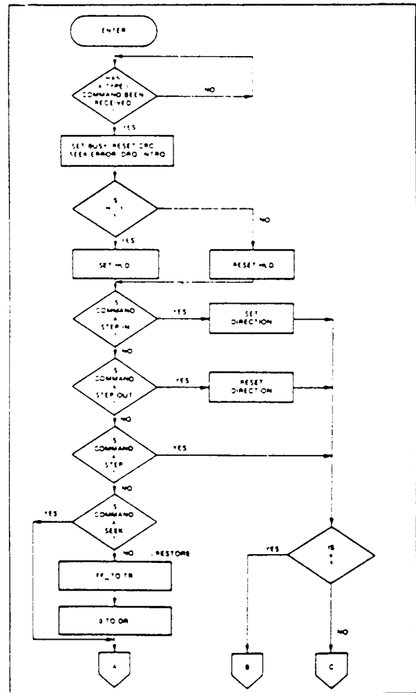
TYPE I COMMAND FLOW
