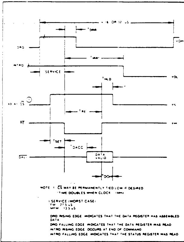
FIGURE 3. READ ENABLE TIMING
