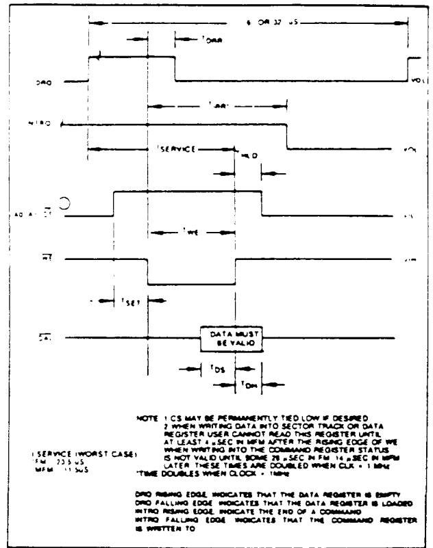
FIGURE 4. WRITE ENABLE TIMING
